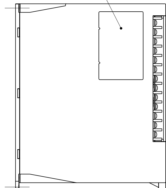
TERMINAL DETAIL
