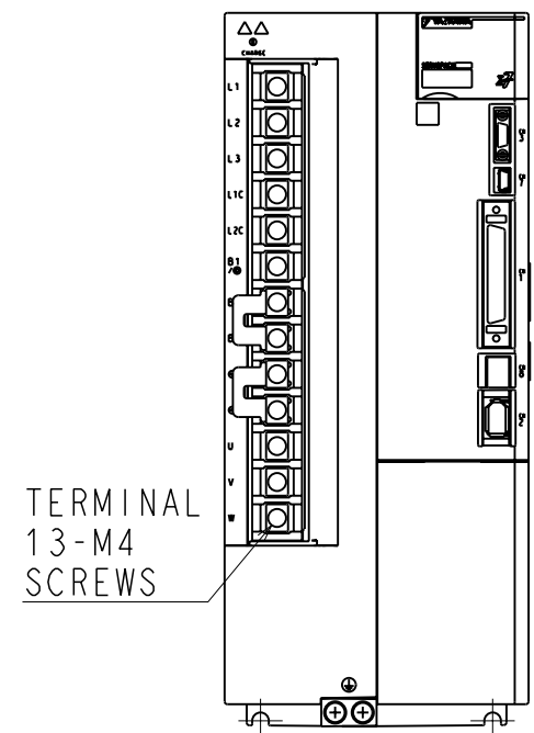
TERMINAL DETAIL
